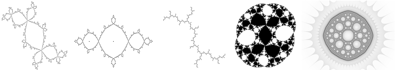
FIGURE 1. Julia sets: rabbit f(z) = z^2 - 0.123 + 0.745i , basilica f(z) = z^2 - 1 , dendrite f(z) = z^2 + i , basilica mated with rabbit f(z) = \frac{z^2+c}{z^2-1} for c = \frac{1+\sqrt{-3}}{2} with J(f) being the boundary between white and black, Sierpiński-Julia carpet f(z) = z^2 - 1/16z^2 i.e. boundaries of Fatou components do not touch each other.
